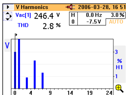
Figure 2. Graph harmonics for voltage and current
