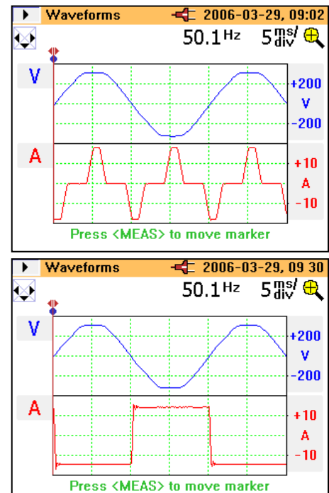
Figure 1. The dual waveform display on the Fluke 345 shows both voltage and current waveforms.
