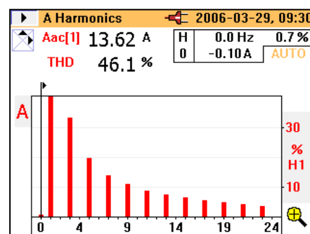
Figure 6. Current harmonics bar graph
