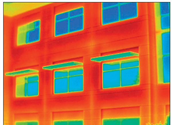
Thermal imaging cameras can identify thermal anomalies within new or existing buildings.
