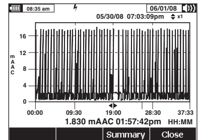
Figure 2. Single refrigeration cycle.
