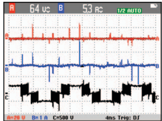
Figure 1. Shaft voltage, common-mode current, and motor drive output displayed on a Fluke 190 Series II ScopeMeter®.
